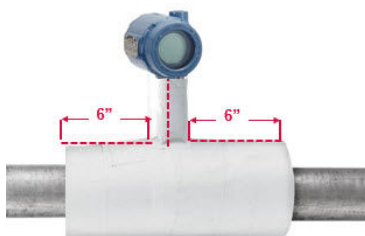
Figure 5-1: Transmitter with Rosemount X-well Technology installation
